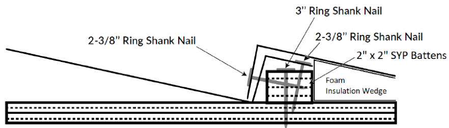
Figure 6 – Attachment Method 2 – Hurricane Metal Shake
